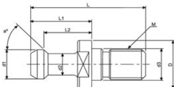
THREAD GROUND
