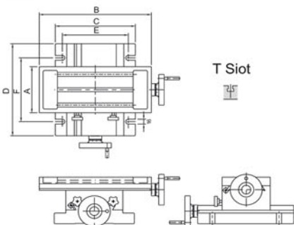
DRAWING OF VCT-514
