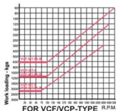
THE CHART FOR LOADING WEIGHT WITH R.P.M.
