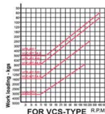
THE CHART FOR LOADING WEIGHT WITH R.P.M.
